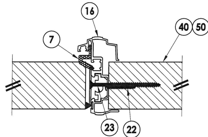
4 HORIZONTAL CROSS SECTION 3 Inswing Shown (Outswing Similar)
