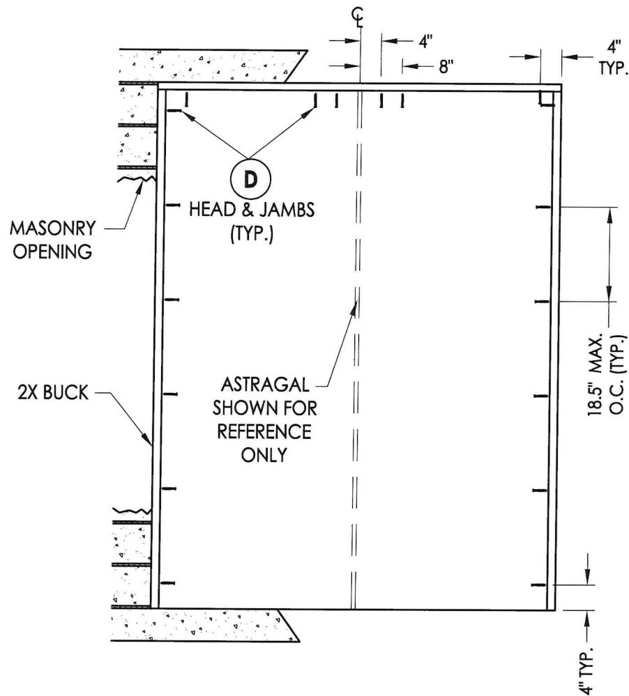
BUCK ANCHORING
