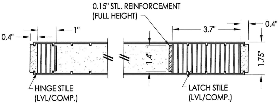
SECTION C-C
