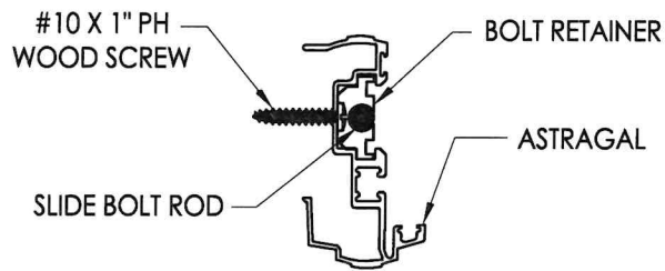
SECTION A-A Astragal Assembly
