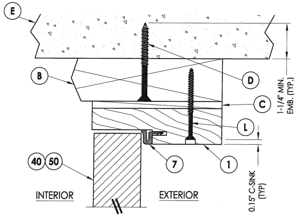
1 VERTICAL CROSS SECTION 3 Inswing Shown (Outswing Similar)
