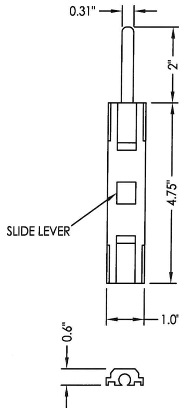
SLIDE BOLT ASSEMBLY w/ Slide Lever (PVC)
